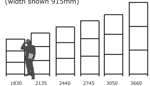
Available Heights (mm) (width shown 915mm)
