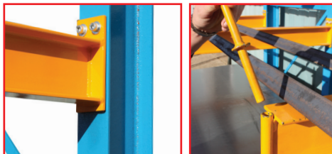
Heavy duty, height adjustable arms with removable end stops
