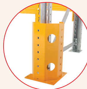
L-Shaped Upright Protector
