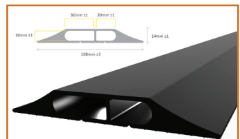
CablePRO Data CP010011 & CP010004 2 x Channel Size: 30mm W x 10mm H & 20mm W x 10mm H
