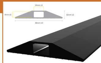
CablePRO GP - Black CP010012 & CP010005 Channel Size: 8mm W x 14mm H
