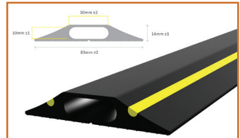
CablePRO GP - Black/Yellow CP010712 & CP010702 Channel Size: 30mm W x 10mm H
