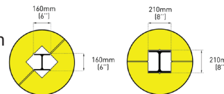
Protector - CP300
